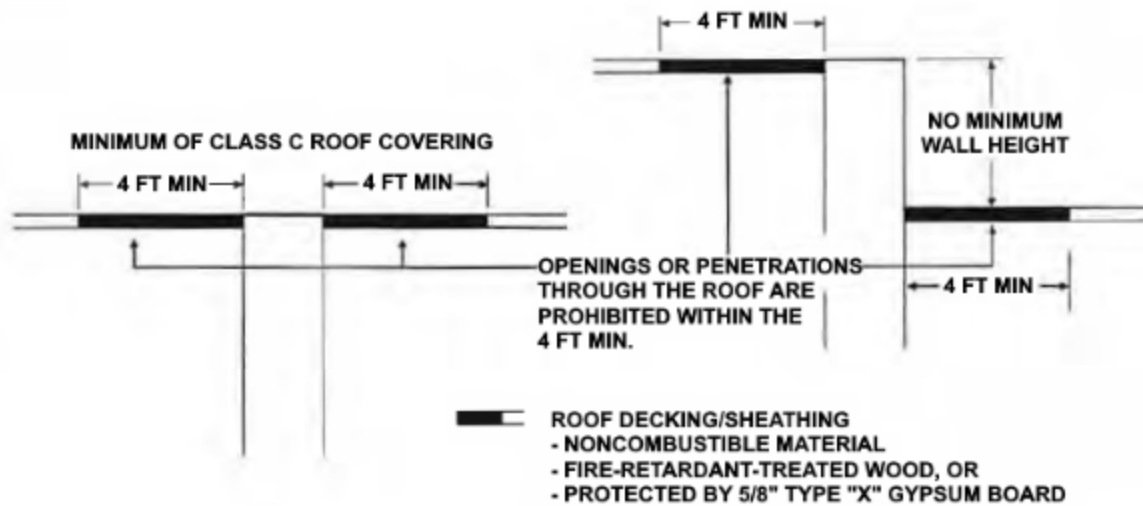
Figure R302.2.2(2) EXCEPTION TO ELIMINATE PARAPET BETWEEN TOWNHOUSES
